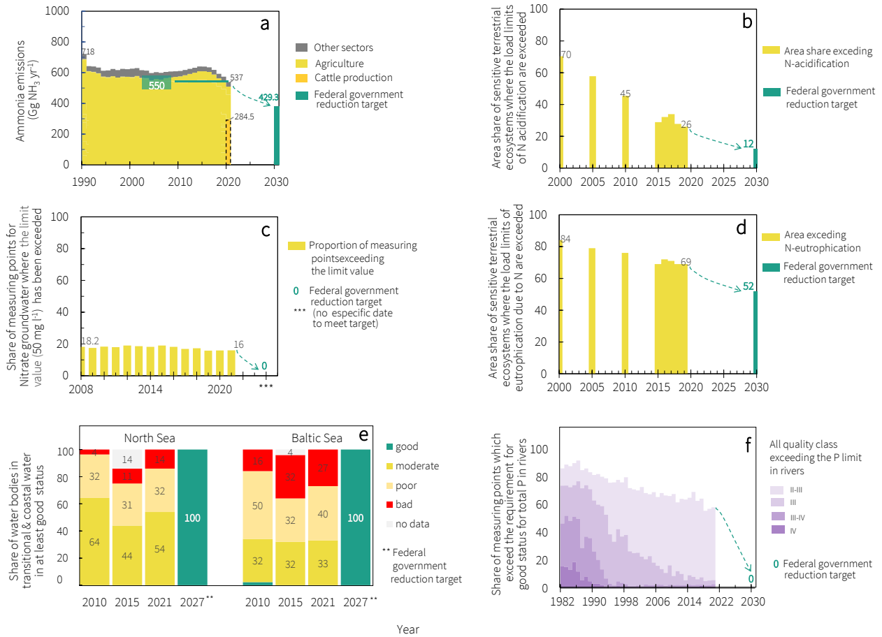
Figure 1: Status of key Nitrogen (N) and Phosphorus (P) pollution indicators for Germany. a. Ammonia emissions: total national and agriculture (1990-2020), cattle primary level of production-related (2020) with discrimination of emission origin, and national reduction target (2010-2020 and 2030); b. Area share of sensitive terrestrial ecosystems where the load limits of acidification are exceeded, several years between 2000 and 2019, reduction target, 2030. c. Share of measuring points for Nitrate groundwater where the limit value ( 50 \text{ mg l}^{-1} ) has been exceeded, modeled development, 2008-2020, reduction target with no date specified. d. Area share of sensitive terrestrial ecosystems where the load limits of eutrophication are exceeded, modeled development, several years between 2000 and 2019, reduction target, 2030. e. Share of transitional and coastal water bodies in at least good status; 2010, 2015, 2021, and reduction target to 2027. Annual data refers to the year of reporting to the EU. When reporting for the year 2010, information was gathered up until 2008. The data for the 2015 reporting year covered the time frame 2009-2014 and for 2021, 2014-2019. f. Share of measuring points that exceed the requirement for good status for total P in rivers, 1982-2021 and reduction target 2030. Color intensity shift from II-III to IV shows worsening status. Data sources: a, national, agriculture related, and reduction target, Vos et al. (2022); cattle-related, calculated in a previous own independent study. b, d, Schaap et al. (2023). c, e, f, Umweltbundesamt (2022).
